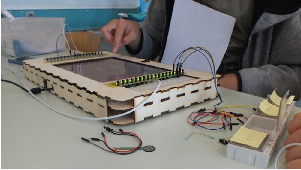
Fig. 11. User study in the Flowboard condition. The participant is seen creating a program to control a piezo buzzer with an acceleration sensor in task 2.
