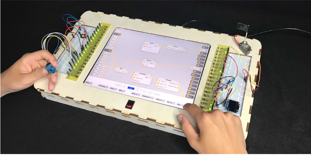
Fig. 1. Flowboard is a system to learn embedded coding based on the flow-based programming (FBP) paradigm. Its hardware combines a large iPad Pro with an Arduino and switchboard circuit beneath it and a breadboard on each side. The user develops her code using Flowboard’s visual FBP editor on the iPad. Electronic components for sensing (input, left) and actuation (output, right) are plugged into the breadboards and linked seamlessly to processing nodes on the screen via two duplicate rows of I/O pins next to the iPad. Parallel processes are easy to code: Here, a physical button (top left) controls what is written to a serial OLED display (bot. right), a force sensor (left center) dims an LED (right center), an on-screen slider (top center) controls a servo, and a 3-axis accelerometer (bot. left) is connected just to see its sensor values live (bot. left).
