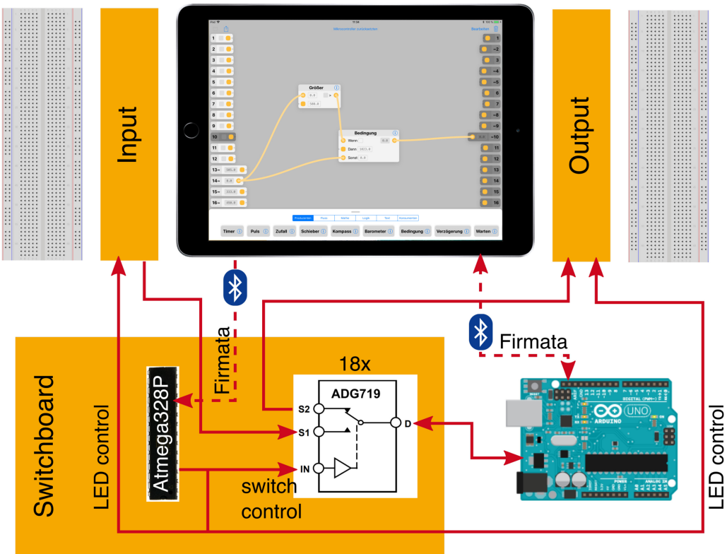
Fig. 3. Flowboard system architecture. The Arduino pins are brought out to the input and output side of the Flowboard via the switchboard, which controls the connection to either side. The iPad runs the visual flow-based editor, and communicates with both the Arduino and the switchboard via Bluetooth using the Firmata protocol [11].
