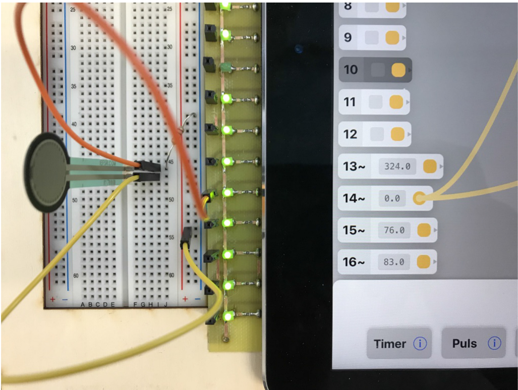
Fig. 7. Close-up of a force sensor connected as input to pin 14. Unlike the other analog pins (13, 15, 16), pin 14 is not floating anymore because it is connected to a defined voltage level. Pins 17 and 18 are currently hidden by the menu in the editor. When the menu is closed, they become accessible again. This example is from a programming task, and shows connections from pin 14 to two different nodes in the editor, as used in Figure 6.
